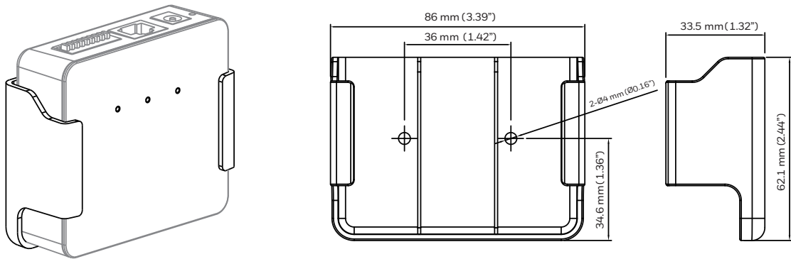
Base Bracket
