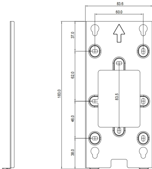
1 FRONT VIEW
