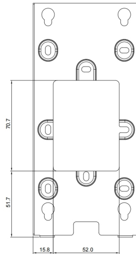
4 BACK VIEW
