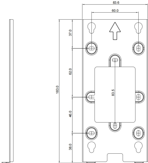
1 FRONT VIEW
