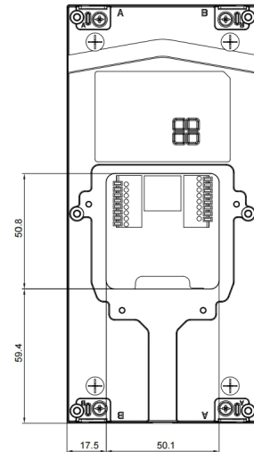
4 BACK VIEW
