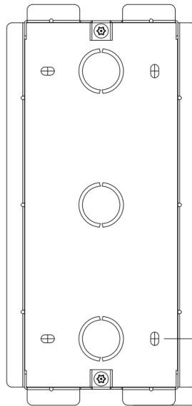
2 FRONT VIEW: FLUSHING MOUNTING BOX PLACEMENT
