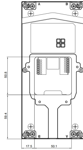
4 BACK VIEW
