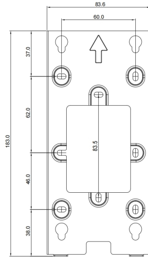
1 FRONT VIEW
