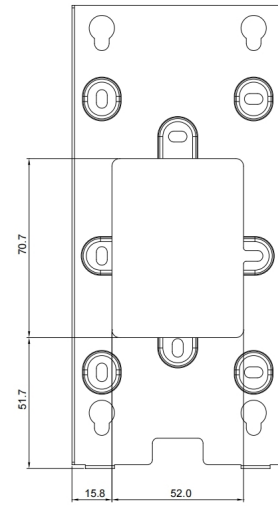
4 BACK VIEW
