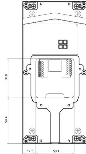
4 BACK VIEW
