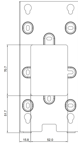
4 BACK VIEW
