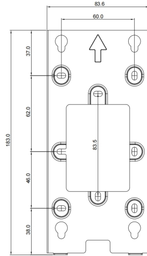
1 FRONT VIEW
