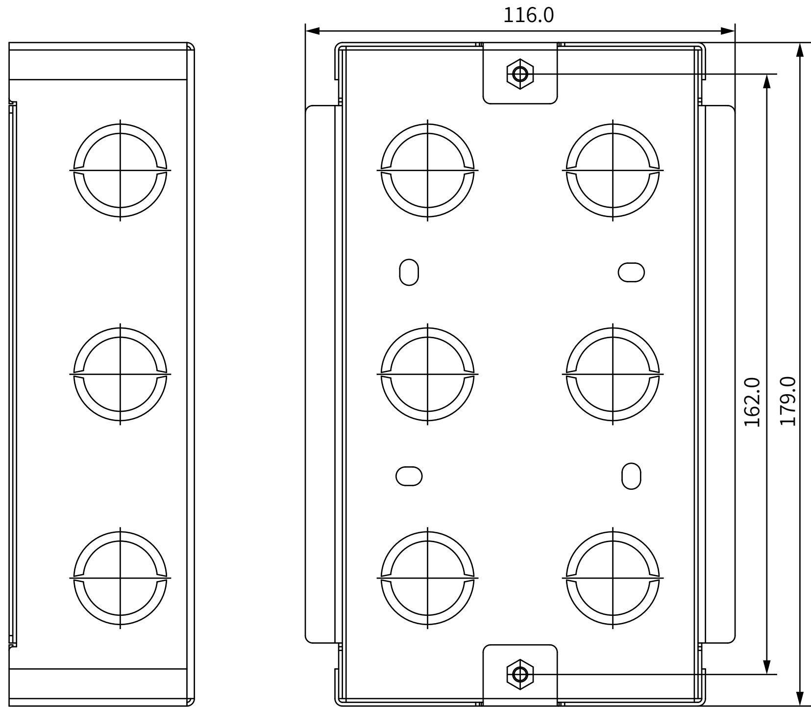
① FRONT VIEW
